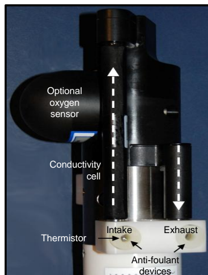
Figure 3: Internal flow path on the HydroCAT.
