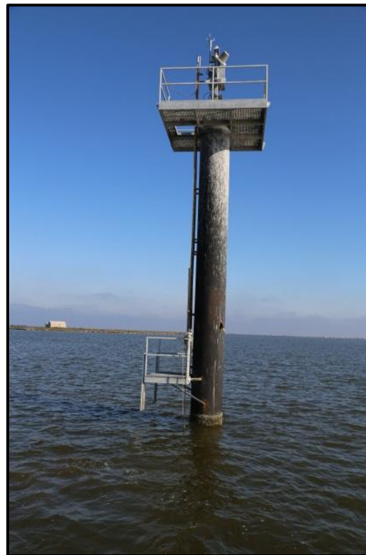
Figure 1a: Sea-Bird Coastal HydroCAT deployment location at Caillou Lake, near Houma, LA
