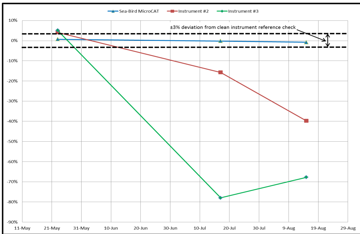
Figure 4: Deviation from clean instrument specific conductivity measurements for three in-situ water quality instruments deployed at Caillou Lake measurement site, summer 2012.
