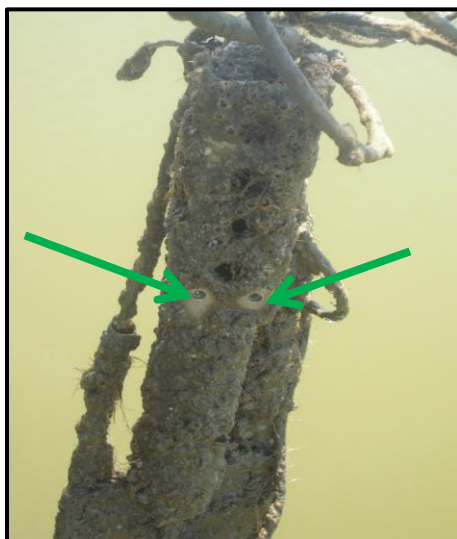
Figure 2: HydroCAT exterior after first visit recovery showing clear intake and exhaust ports.
