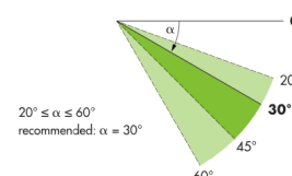
Figure 3: OTT SVR 100 instrument alignment
