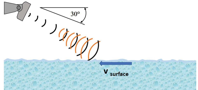
Figure 2: OTT SVR 100 velocity measuring principle
