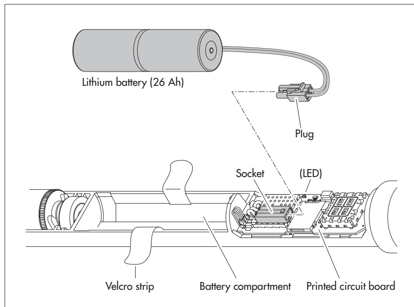
Fig. 3: Inserting the lithium battery.
