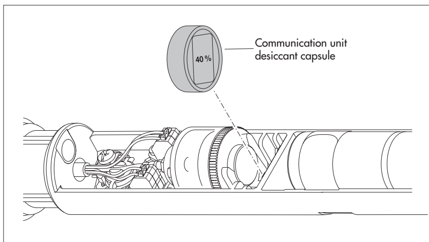
Fig. 21: Replacing the communication unit desiccant capsule.
