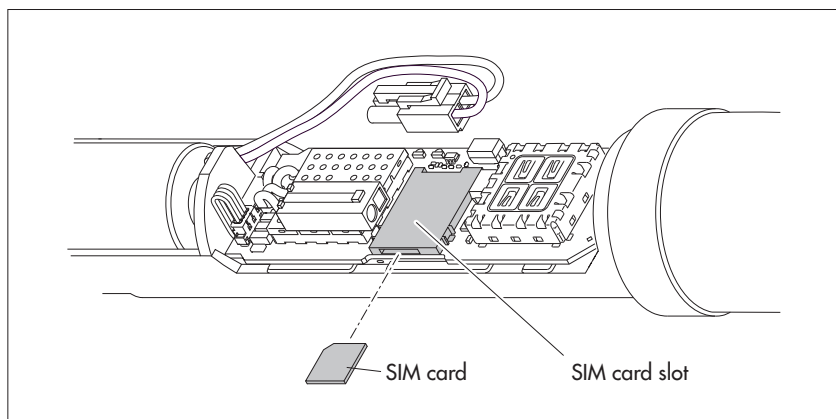
Fig. 4: Inserting the SIM card.
